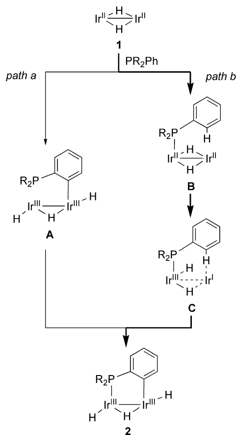
Scheme 2. Plausible reaction pathways for the oxidative addition of a C-H bond to 1 induced by the coordination of a phosphorus ligand.
