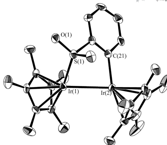
Figure 4. ORTEP drawing of complex 6a with 50% thermal probability ellipsoids. Hydrogen atoms are omitted for clarity. Selected bond lengths [Å] and angles [°]: Ir(1)–Ir(2) 2.9836(2), Ir(1)–S(1) 2.2034(15), Ir(2)–C(21) 2.055(5), S(1)–C(22) 1.790(6), S(1)–O(1) 1.485(4), Ir(2)–Ir(1)–S(1) 80.08(3), Ir(1)–Ir(2)–C(21) 83.98(13).
