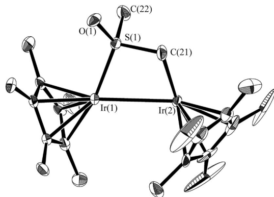
Figure 3. ORTEP drawing of complex 5 with 50% thermal probability ellipsoids. Hydrogen atoms are omitted for clarity. Selected bond lengths [Å] and angles [°]: Ir(1)–Ir(2) 2.9414(4), Ir(1)–S(1) 2.2097(19), Ir(2)–C(21) 2.112(9), S(1)–C(21) 1.739(10), S(1)–C(22) 1.797(9), S(1)–O(1) 1.485(6), Ir(2)–Ir(1)–S(1) 71.26(5), Ir(1)–Ir(2)–C(21) 74.0(2).
