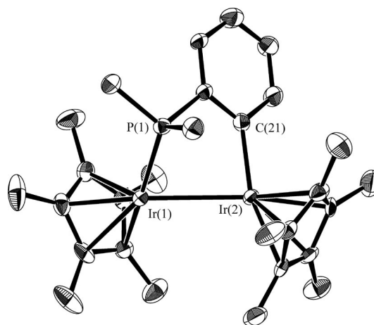
Figure 1. ORTEP drawing of complex 2a with 50% thermal probability ellipsoids. Hydrogen atoms are omitted for clarity. Selected bond lengths [Å] and angles [°]: Ir(1)–Ir(2) 2.9782(4), Ir(1)–P(1) 2.214(2), Ir(2)–C(21) 2.052(8), Ir(2)–Ir(1)–P(1) 76.83(5), Ir(1)–Ir(2)–C(21) 84.7(2).
