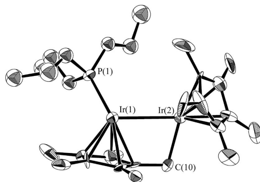
Figure 2. ORTEP drawing of complex 4 with 50% thermal probability ellipsoids. Hydrogen atoms are omitted for clarity. Selected bond lengths [Å] and angles [°]: Ir(1)–Ir(2) 2.9315(19), Ir(1)–P(1) 2.179(7), Ir(2)–C(10) 2.14(2), Ir(2)–Ir(1)–P(1) 113.5(7), Ir(1)–Ir(2)–C(1) 76.2(10).
